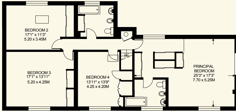
FIRST FLOOR 1232 SQ.FT.
