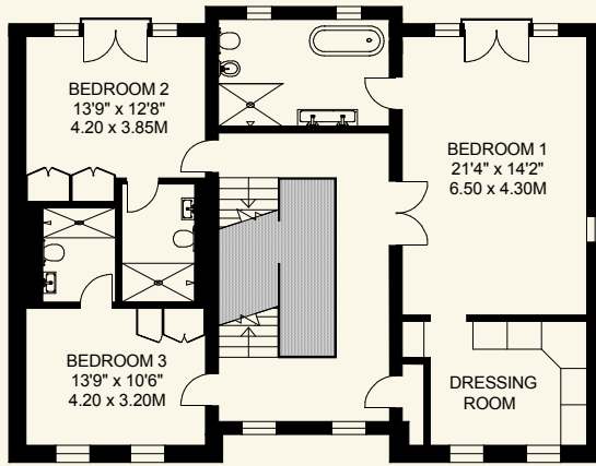
FIRST FLOOR 1242 SQ.FT.
