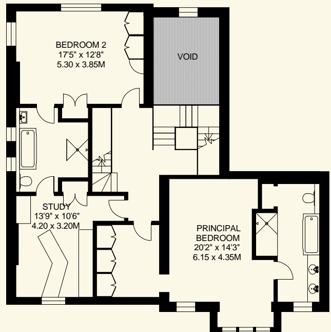
FIRST FLOOR 1200 SQ.FT.
