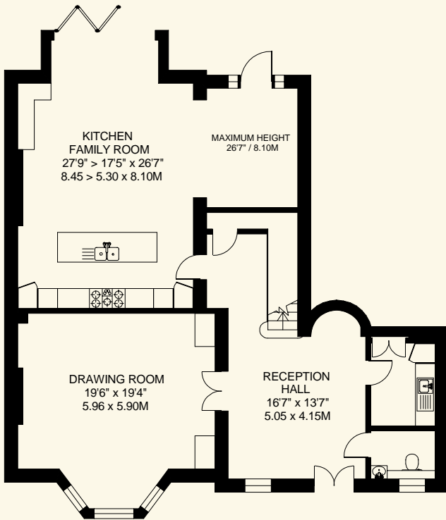
GROUND FLOOR 1340 SQ.FT.
