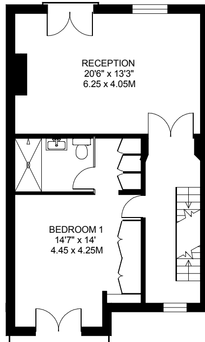
FIRST FLOOR 682 SQ.FT.
