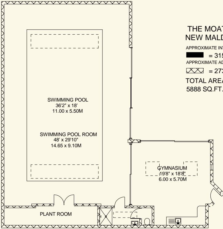
GROUND FLOOR 1953 SQ.FT.
